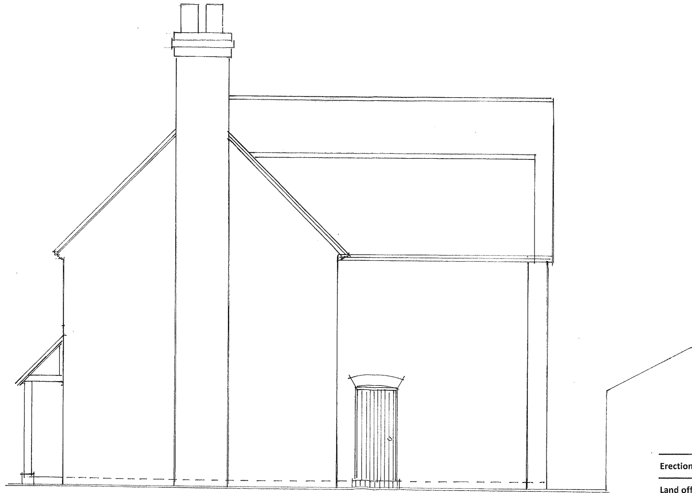
East Elevation
